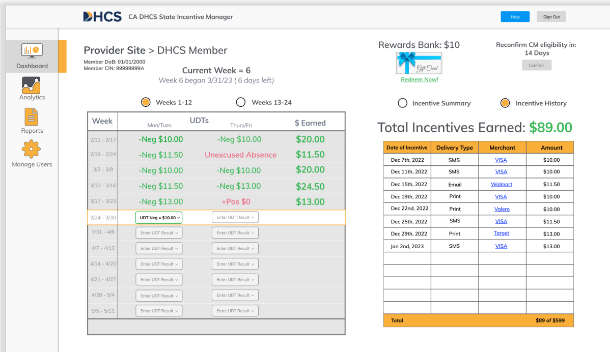
Figure 5. Member Pane
